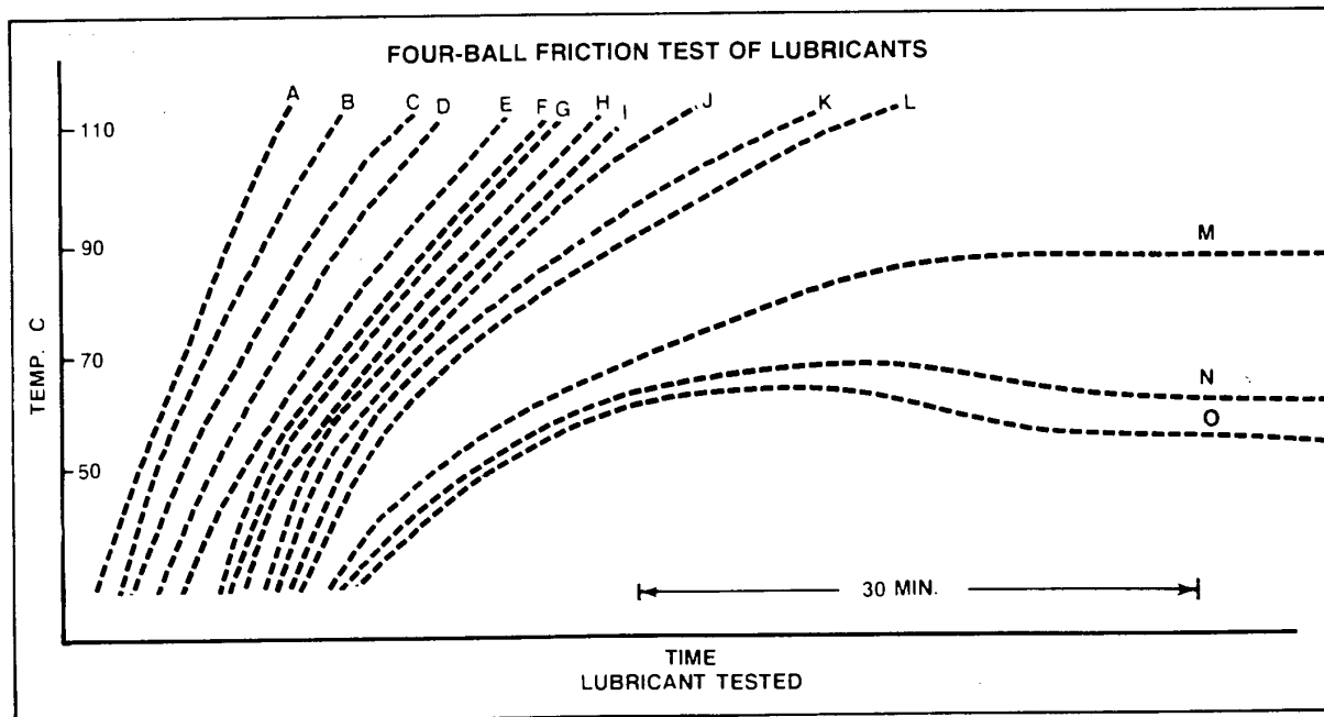
3/8" DIAMETER STEEL BALLS AMBIENT 24°C CODE 20-336
