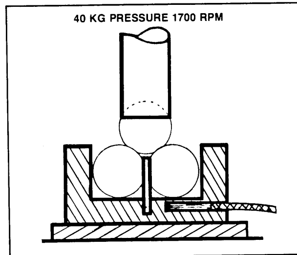
3/8" DIAMETER STEEL BALLS AMBIENT 24°C CODE 20-336
