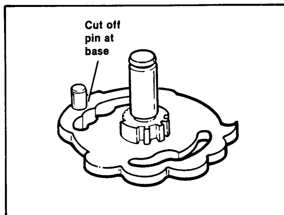
Gear Shifter Cam
