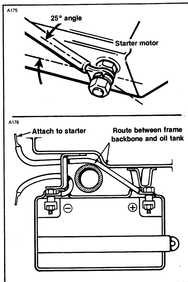
Figure 2. Battery Cable Routing
