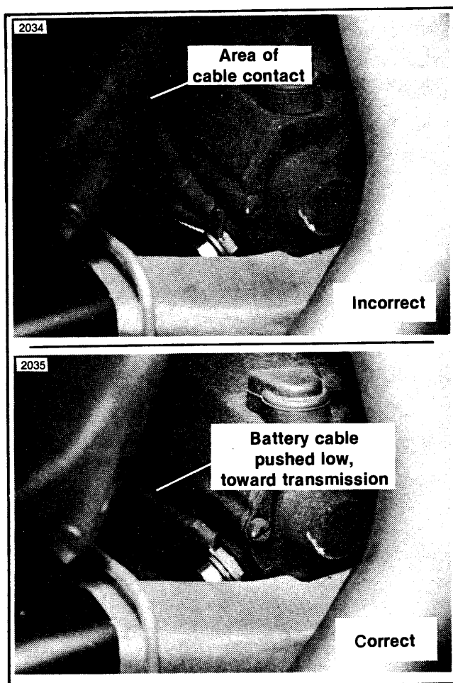
Figure 1. Connection to Starter
