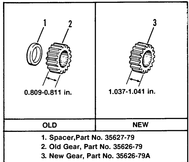
Figure 1. Old and New 5th Gears, Countershaft
