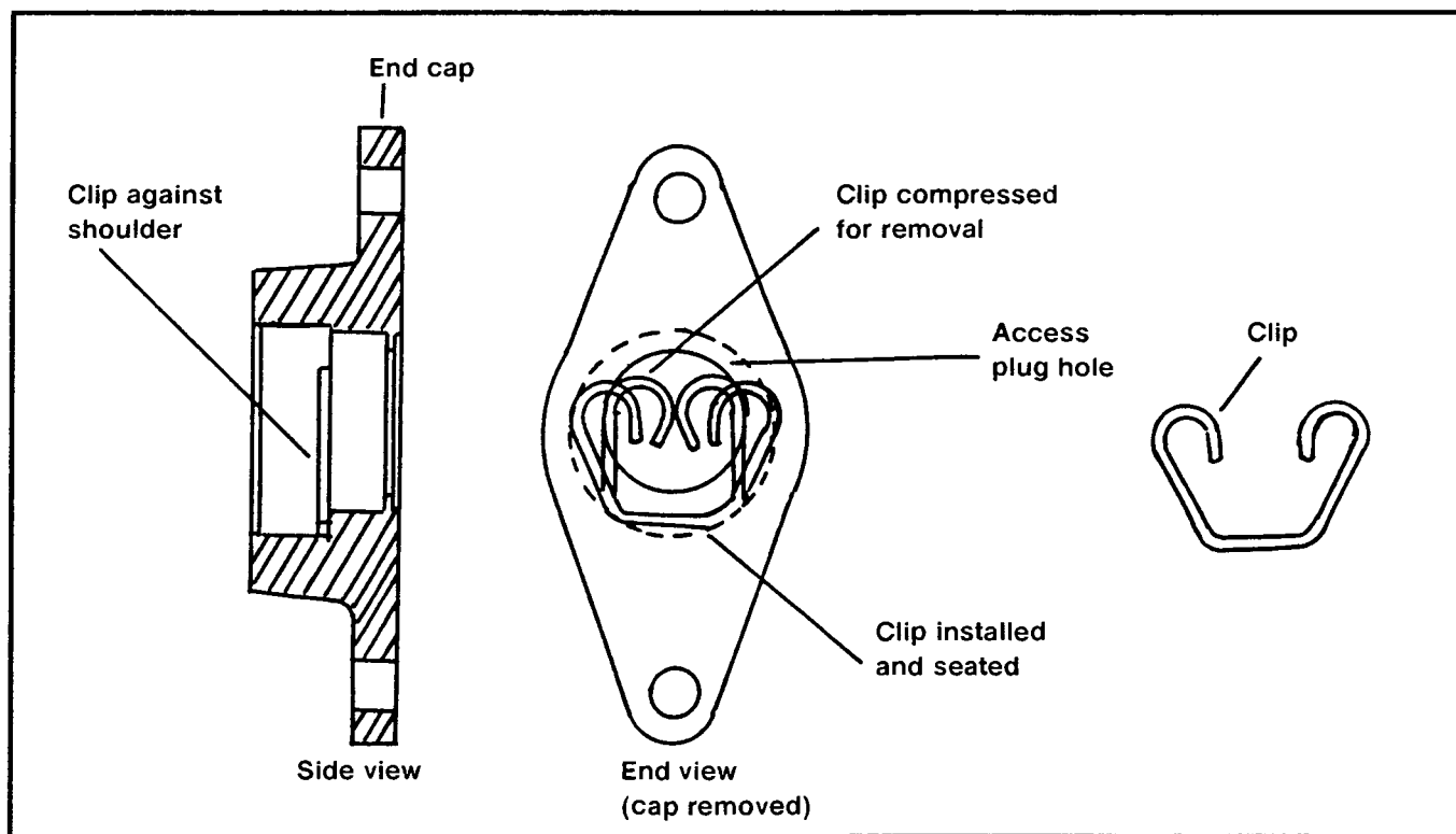
Figure 1. Retaining Clip Installation
