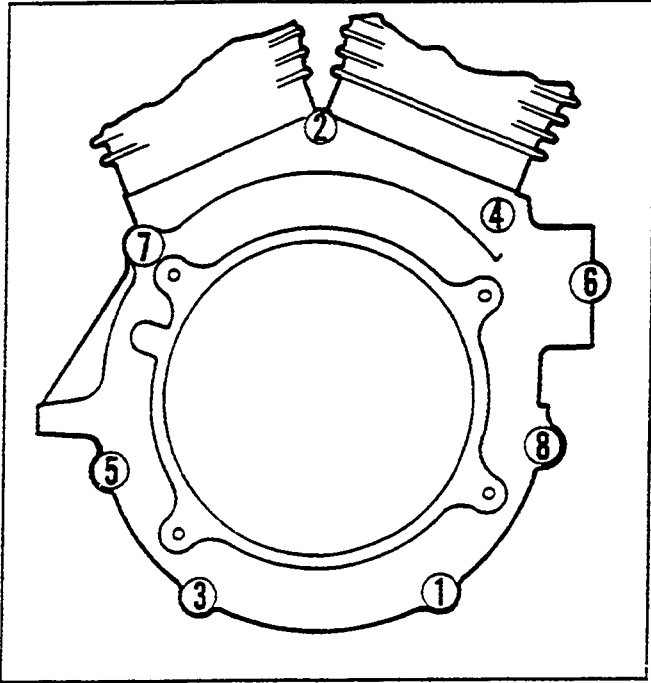
Figure 5. Crankcase Torque Sequence
