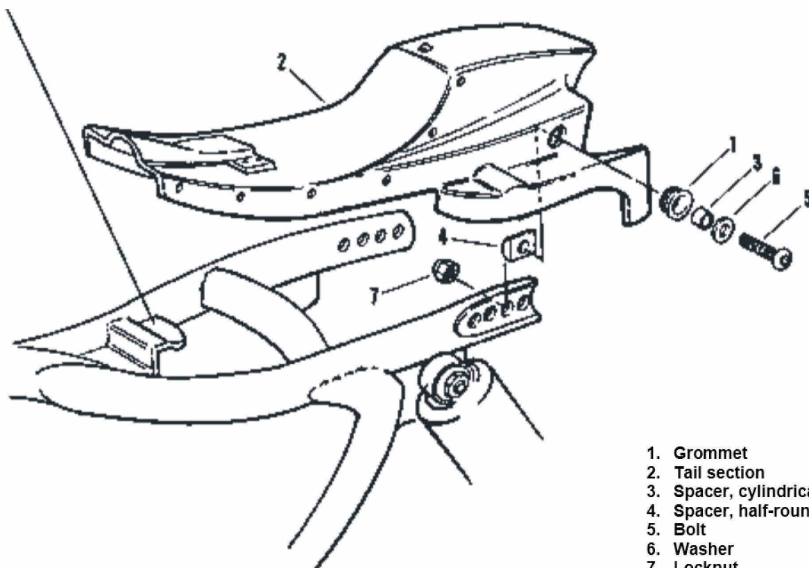
Tail Section Bracket Assembly
