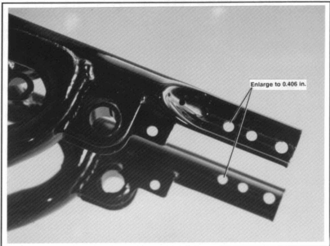
XL Frame assembly
