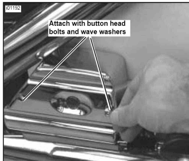
Figure 3. Attach chrome cover with wave washers and button head bolts.
