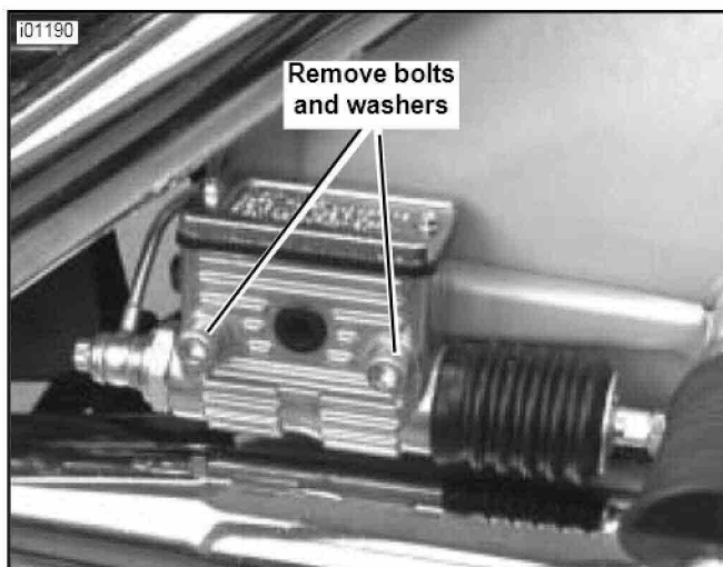
Figure 1. Remove bolts and washers shown
