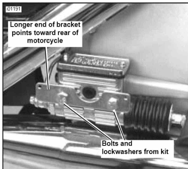
Figure 2. Mounting plate position
