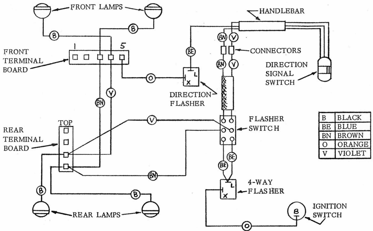
WIRING DIAGRAM
